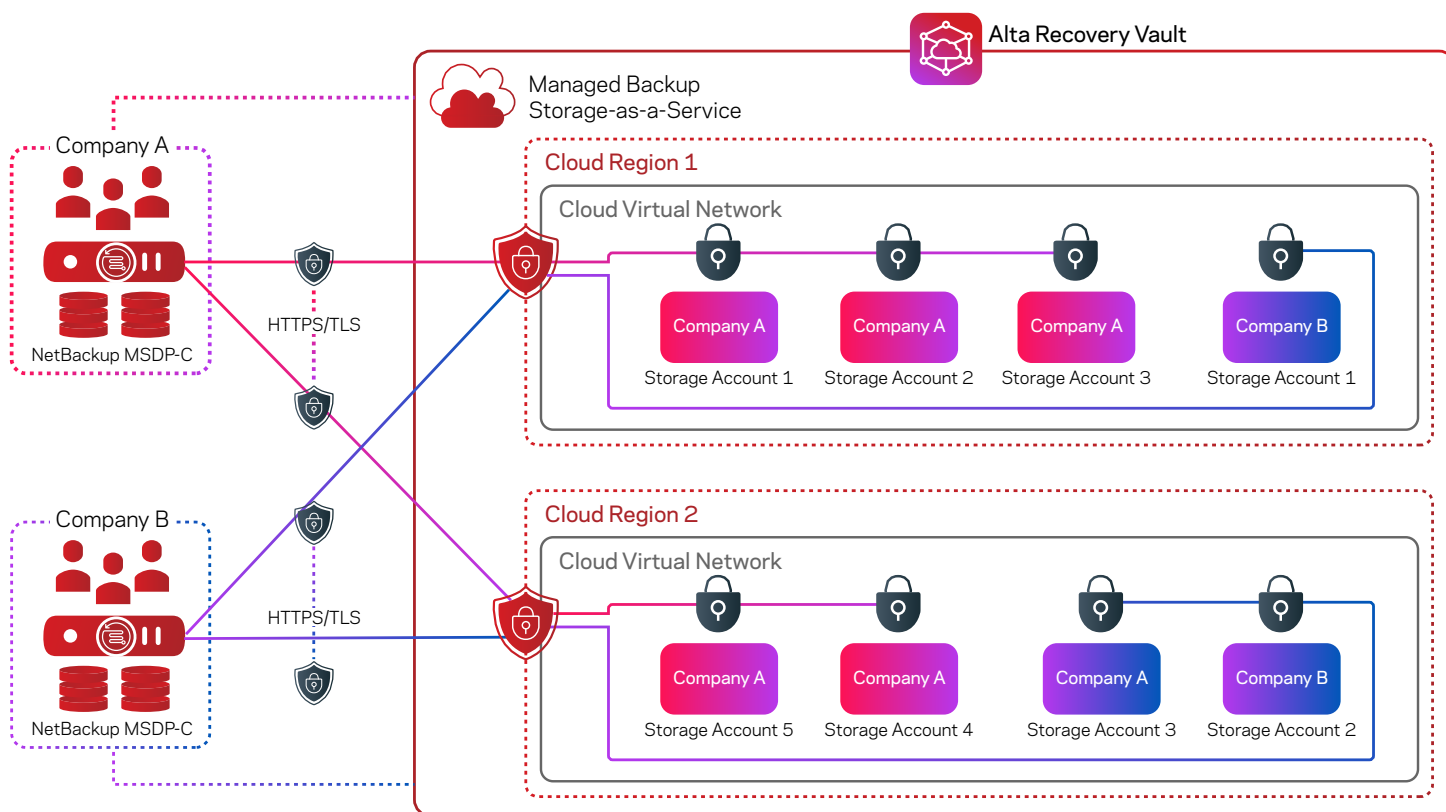
Figure 11. Veritas Alta Recovery Vault architecture overview
